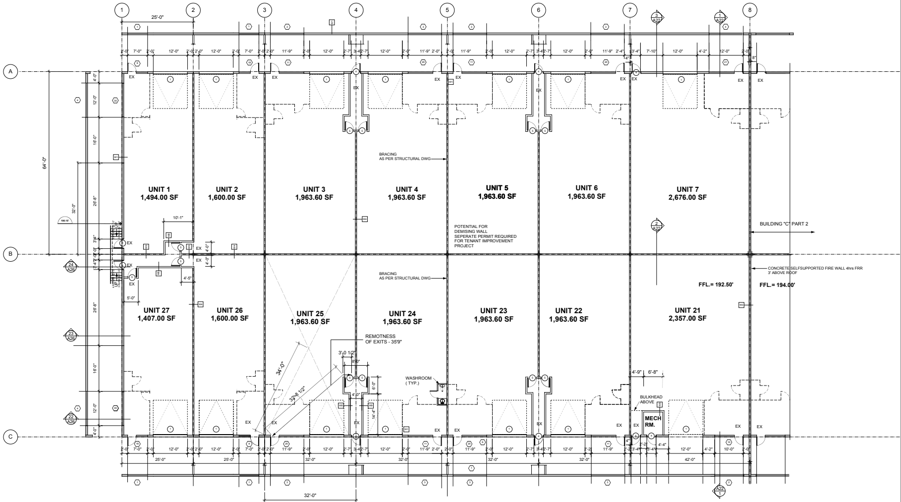
BUILDING "C" - LEVEL 1, PART 1
